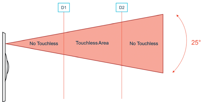
Activation range of the touchless function D1 = typ. 25 mm, D2 = typ. 85 mm
